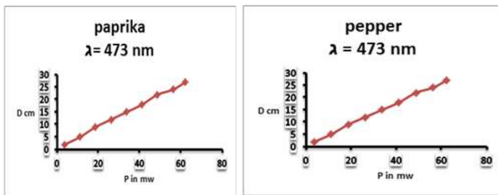
Fig (9):Variation of external ring diameter against input power at \lambda = 473 \text{ nm} for paprika oil and pepper oil .
