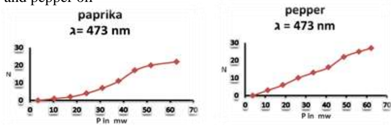
Fig (7):Variation of rings number against input power at \lambda = 473 \text{ nm} for paprika oil and pepper oil.
