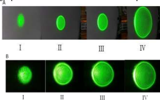
Fig (4). Variation of rings number in (A) paprika oil [ I : 3.8 mW , II: 15.2 mW , III: 30.4 mW , IV: 68.4 mW ] and (B) pepper oil [ I : 7.4 mW , II: 29.6mW , III: 66.6mW , IV: 81.4 mW ] using light beam of \lambda = 532 nm against input power.
