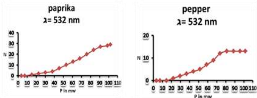
Fig (6):Variation of rings number oil against input power at \lambda = 532 \text{ nm} for paprika oil and pepper oil
