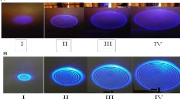
Fig. (5) : Variation of rings number in (A) paprika oil [ I: 3.45 mW , II: 17.25 mW , III: 31.05 mW , IV: 37.95 mW ] and (B) pepper oil [ I: 11.25 mW , II: 26.25 mW , III: 41.25mW , IV: 56.25 mW , ] using light beam of \lambda = 473 nm against input power.
