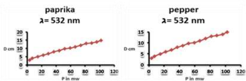
Fig (8):Variation of external ring diameter against input power at \lambda = 532 \text{ nm} for paprika oil and pepper oil .
