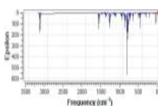
Coronene-Cl
