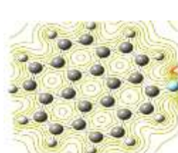
Coronene-Cl
