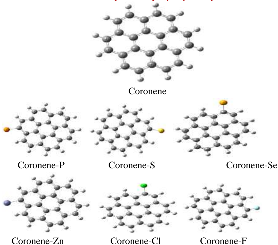
Figure(1) The molecular structure for Coronene and Coronene-Y.
