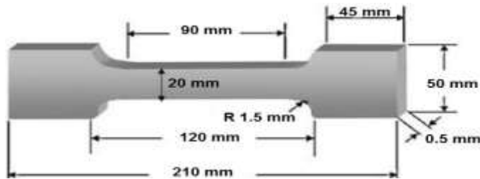
Figure ( 2 ) The shape and dimensions of the specimen used in the current paper[16]
