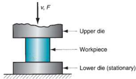
Figure (1) Open-Die Forging
