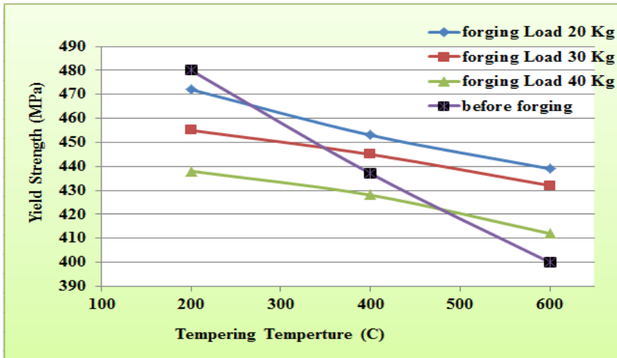
Figure (4) Tempering temperature Vs Yield Strength
