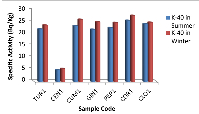
(a) For ^{40}\text{K} nuclide
