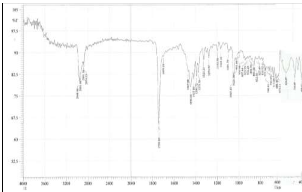
Figure (3): IR spectra for complex 2
