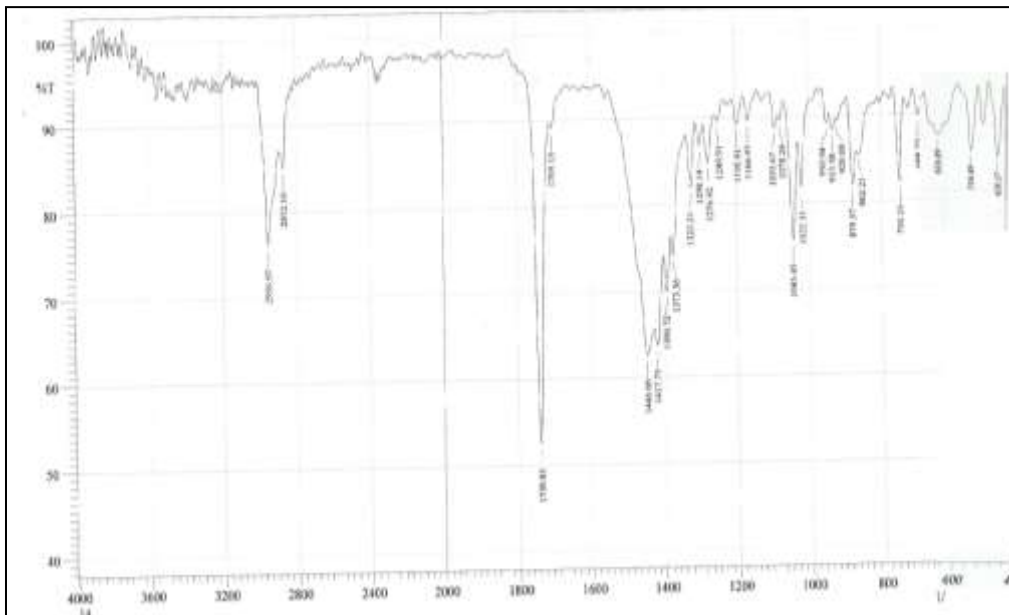
Figure (5): IR spectra for complex 4
